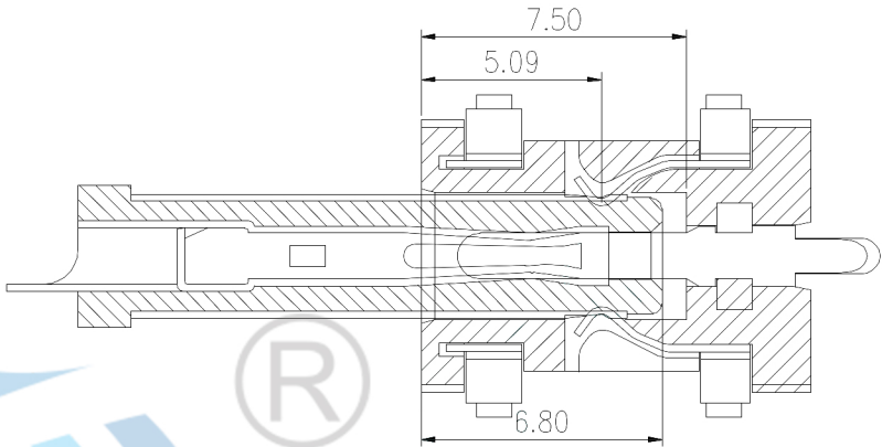
DC JACK INSERT DEPTH
