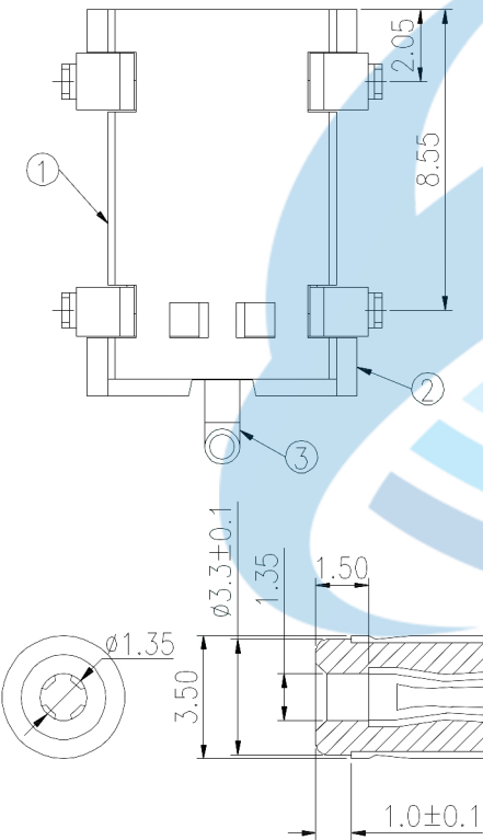
DC MATE PLUG
