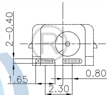
P.C.B LAYOUT (front view)
