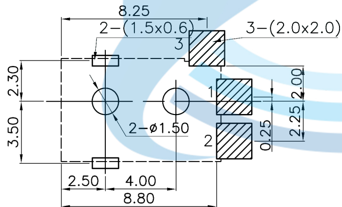
P.C.B LAYOUT(Copper-side view)
