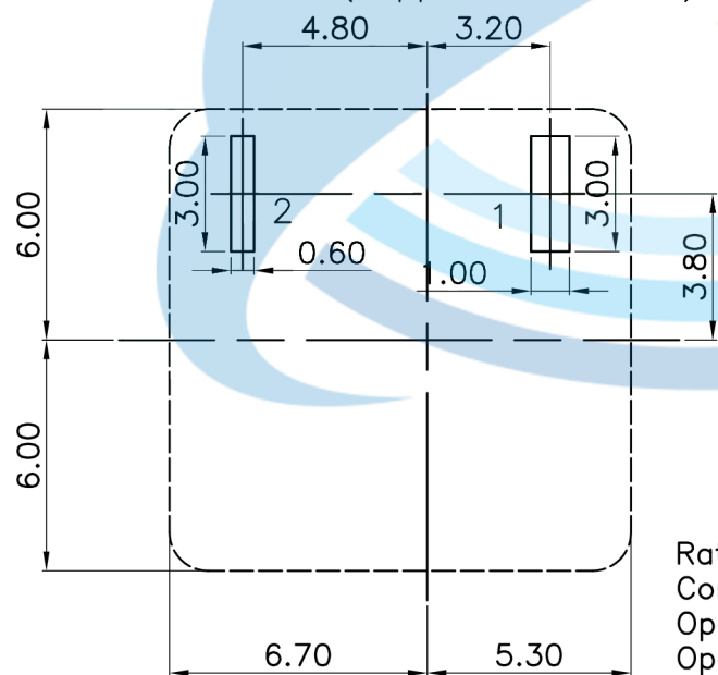
P.C.B LAYOUT(copper-sided view)
